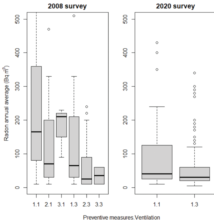
Fig. 5. Boxplot showing the effect of building regulations of 2010 and the required preventive radon measures on annual average indoor ^{222}\text{Rn} concentration. Figure legends on x-axis: 1.1: knowledge of installed measures and having other ventilation than balanced; 2.1: having knowledge of no installed measures and having other ventilation than balanced; 3.1: not knowing about installed measures and having other ventilation than balanced; 1.3: knowledge of installed measures and having balanced ventilation; 2.3: having knowledge of no installed measures and having balanced ventilation; 3.3: not knowing about installed measures and having balanced ventilation.
