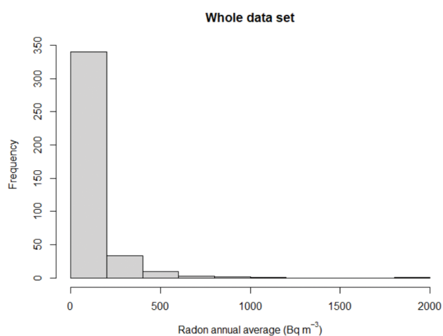
Fig. 1. Histogram of all ^{222}\text{Rn} concentration measurements.
