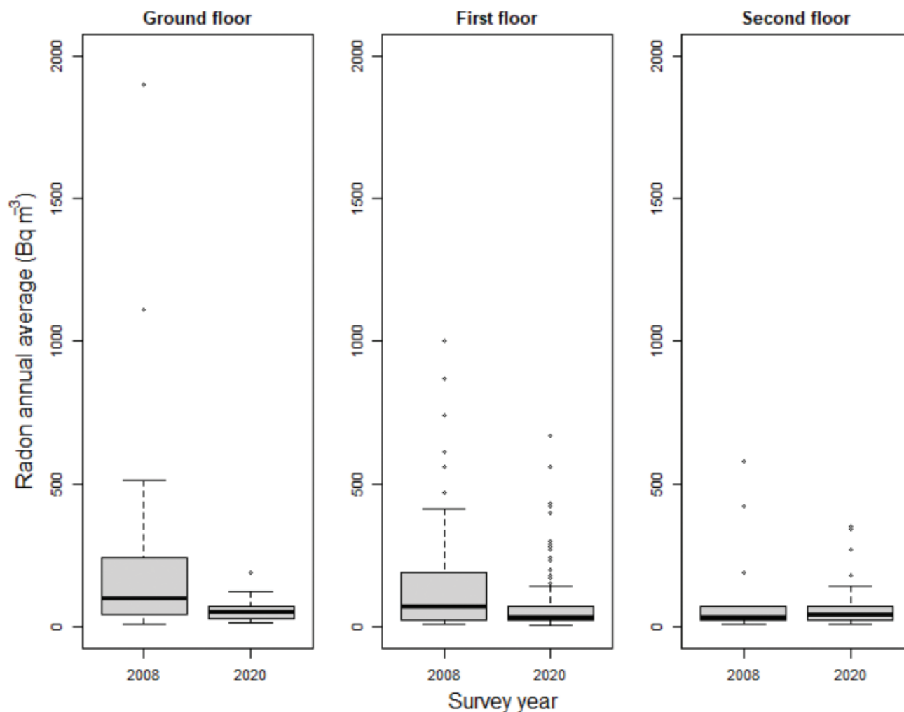
Fig. 3. Boxplot of annual average indoor ^{222}\text{Rn} concentration per floor for the two surveys.
