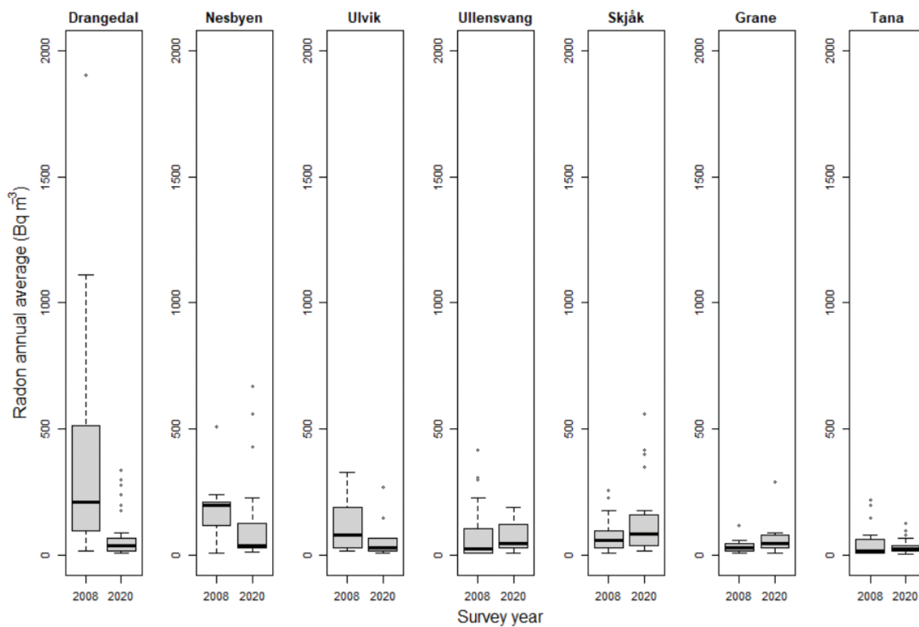
Fig. 4. Boxplot of annual average indoor ^{222}\text{Rn} concentration per municipality for the two surveys.
