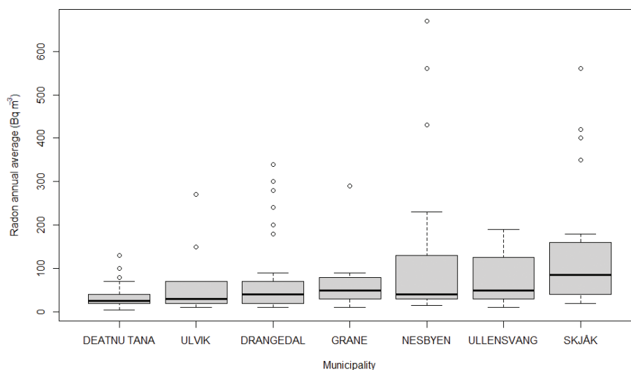
Fig. 6. Boxplot of annual average indoor ^{222}\text{Rn} concentration per municipality in the 2020 survey.
