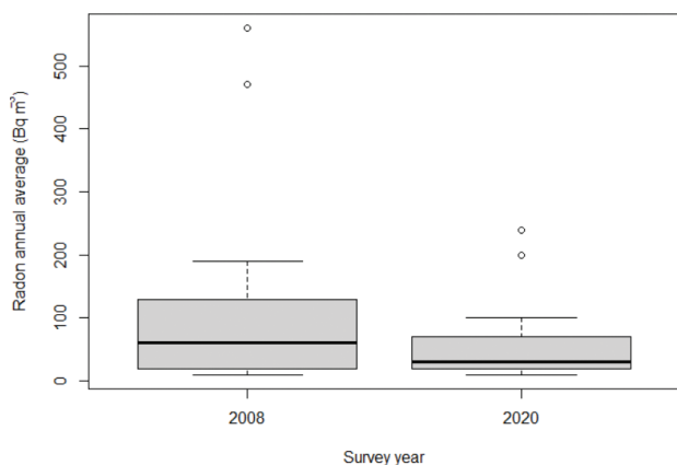
Fig. 2. Boxplot of annual average indoor ^{222}\text{Rn} concentration measurements for the 18 homes with crawl space.
